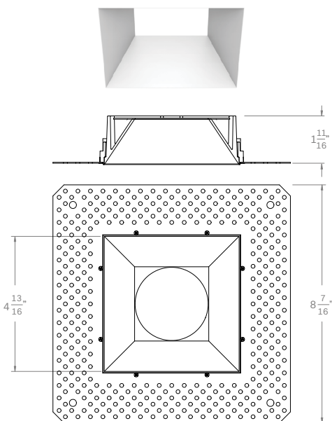
STL 4" Acrobat Square Trimless Mud Plate (with Standard Reflector)
