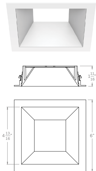
SST 4" Acrobat Square Standard Trim (with Standard Reflector)
