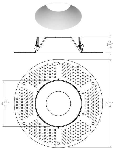
RTL 4" Acrobat Round Trimless Mud Plate (with Standard Reflector)
