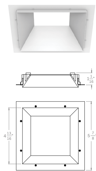
SWC 4" Acrobat Square Wood Ceiling Trim (with Standard Reflector)
